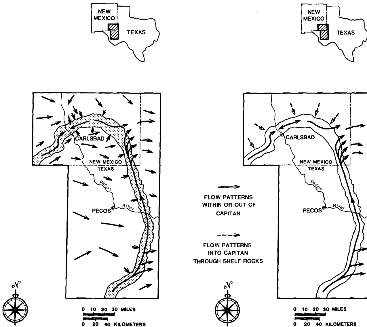
Figure V-2. Comparison of Models Proposed for Groundwater Movement in Guadalupian Rocks of the Delaware Basin. Arrows indicate relative magnitudes and directions of groundwater flow. Note no involvement of the "basin aquifer" and a greater involvement of the "shelf aquifer" in B.
