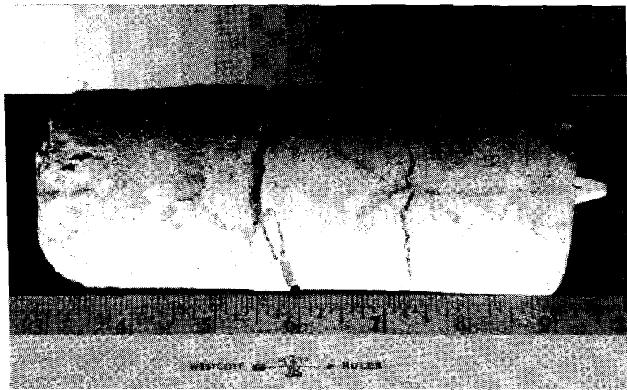
Figure VIII-4. Photograph, Core From Marker Bed 103 (WIPP 25) Containing Halite-Filled Fractures
